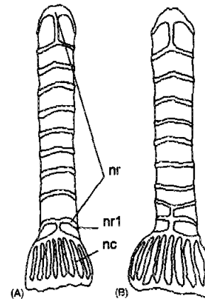
Fig. 6. Dorsal view of nasal skeleton of (A), some Paramyxine nelsoni and (B), P. yangi and some P. nelsoni . nc, nasal capsule; nr, nasal ring; nr1, 1st nasal ring.
